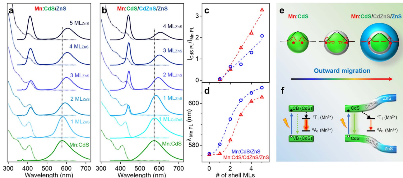
Fig. 2 (a and b) Normalized absorption (dotted lines) and PL (solid lines) spectra of Mn: CdS/ZnS (1–5 ML ZnS) and Mn: CdS/CdZnS/ZnS (1–4 ML ZnS) core/multi-shell QDs, respectively. (c) The PL intensity ratio of CdS host lattice and Mn(II) and (d) the changes of Mn(II) PL peak position as a function of ZnS and CdZnS/ZnS shell thickness for Mn: CdS/ZnS (1–5 ML ZnS) and Mn: CdS/CdZnS/ZnS (1–4 ML ZnS) core/multi-shell QDs, respectively. (e) Schematic of the dopant outward migration by inserted CdZnS alloyed trap layer and (f) the band alignment of the Mn: CdS/CdZnS/ZnS core/multi-shell QDs.
