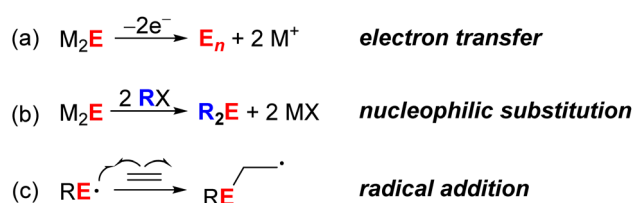
Scheme 1 Examples of chalcogenide-centered reactions (E = S, Se).
