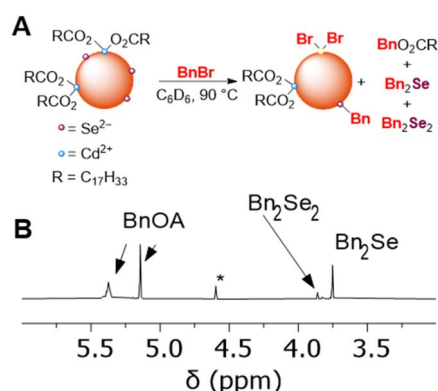
Fig. 7 (A) Scheme showing that benzylation of carboxylate ligands and of surface selenide ions of CdSe QDs upon treatment with benzyl bromide. (B) Truncated 1 H NMR spectrum showing benzylic resonances of a CDCl 3 solution of molecular products formed upon heating a benzene mixture of OA-capped CdSe QDs ( d \sim 3.6 nm, 0.5 mM) and BnBr (50 equiv. per QD) at 90 °C for 15 h. (*) indicates a Bn 2 O impurity.
