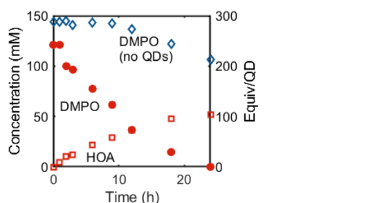
Fig. 6 Concentrations of DMPO (red circles) and oleic acid (red squares) in a C 6 D 6 mixture of OA-capped CdSe QDs ( d \sim 3.6 nm, 0.5 mM) and DMPO (300 equiv. per QD) over time during irradiation ( \lambda = 440 nm, 200 mW cm −2 ). The concentration of a C 6 D 6 solution of DMPO during irradiation ( \lambda = 370 nm, 100 mW cm −2 ) in the absence of QDs is included for comparison (blue diamonds).
