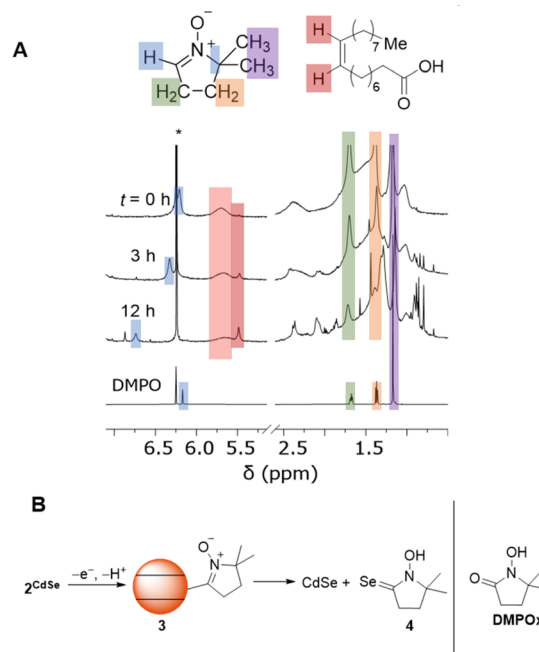
Fig. 5 (A) ^1\text{H} NMR spectra of a \text{C}_6\text{D}_6 mixture of zinc blende OA-capped CdSe QDs ( d \sim 3.6 nm) and DMPO (300 equiv. per QD) during irradiation ( \lambda = 440 nm, 200 \text{ mW cm}^{-2} ). (B) Proposed oxidative formation of DMPO-derived diamagnetic products from 2^{\text{CdSe}} .
