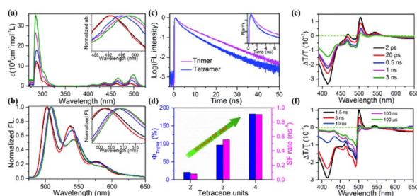
Fig. 14 (a) and (b) Absorption (a) and fluorescence (b) spectra of dimer 4, trimer 40 and tetramer 41 and their corresponding monomers. (c) Triplet yield and SF rate of dimer 4, trimer 40 and tetramer 41. (d) Triplet yield and SF rate of dimer 4, trimer 40 and tetramer 41. (e) and (f) fs- (e) and ns- (f) TA of tetramer 41. Reproduced with permission. 172 Copyright 2018, The Royal Society of Chemistry.
