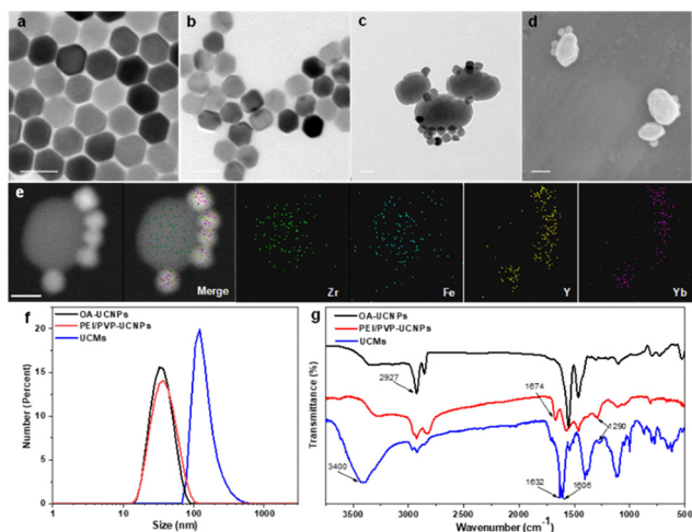
Fig. 1 TEM images of (a) UCNP (NaYF 4 :25% Yb 3+ , 0.9% Tm 3+ , 0.6% Nd 3+ ), (b) dual-ligand PEI/PVP modified UCNP, and (c) UCNP. (d) SEM images of UCNP-MOF heterostructure. (e) Dark-field TEM image and the corresponding area-elemental mapping of UCNP-MOF heterostructure, including Zr, Fe, Y and Yb. (f) The statistical data showing the size distributions of OA-UCNPs, PEI/PVP-UCNPs and UCNP-MOF heterostructures. (g) FT-IR spectra for OA-UCNPs, PEI/PVP-UCNPs and UCNP-MOF heterostructures. The scale bars indicate 50 nm in all the tested cases.
