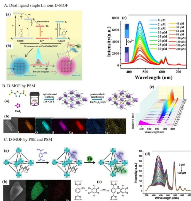
Fig. 13 (A) The design principle and preparation of Eu-DATA/BDC, where \text{H}_2\text{BDC} sensitizes \text{Eu}^{3+} ions to realize the antenna effect emission and \text{DATA} maintains its own emission and identifies \text{Cu}^{2+} ions, and the fluorescence spectra of Eu-DATA/BDC in aqueous solutions with \text{Cu}^{2+} ions at different concentrations. Reproduced with permission from ref. 199. Copyright 2022, Elsevier. (B) Eu-Ca-MOF prepared by PSM. (a) The synthesis of Eu-Ca-MOF. (b) The EDX element mapping diagram of Eu-Ca-MOFs and (c) the emission spectra of Eu-Ca-MOFs after treatment with different metal ions. Reproduced with permission from ref. 212. Copyright 2023, Elsevier. (C) The construction of D-MOFs by PSE. (a) and (b) The synthesis procedure, SEM image, and SEM-EDX elemental mapping of \text{Tb}@ \text{UiO}-66-(\text{COOH})_2\text{NH}_2 . (c) The mechanism of capturing o-TCBQ by \text{atp}^{2-} ligand. (d) The photoluminescence spectra of \text{Tb}@ \text{UiO}-66-(\text{COOH})_2\text{NH}_2-40 at different concentrations of o-TCBQ. Reproduced with permission from ref. 220. Copyright 2016, the American Chemical Society.
