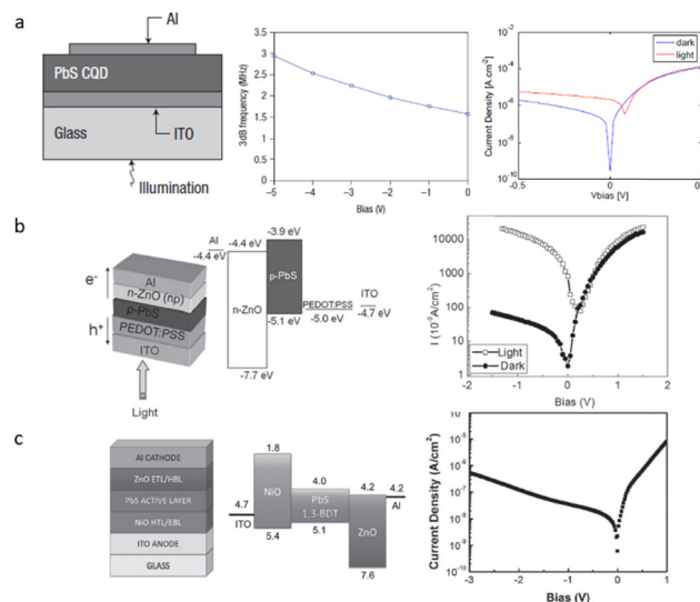
Fig. 9 (a) A schematic of the PbS CQD photodiode, frequency dependence (3 dB) on bias, and steady-state I-V characteristics in the dark and at 17.9 \mu\text{W cm}^{-2} illumination at 1550 nm. Reprinted with permission from ref. 99. Copyright 2008, Springer Nature Limited. (b) Device structure of ITO/PEDOT:PSS/PbS-NQD/ZnO/Al photodiode; its energy band diagram and the I-V characteristics in dark and under 200 \mu\text{W cm}^{-2} illumination at 500 nm. Reprinted with permission from ref. 100. Copyright 2012, John Wiley & Sons, Inc. (c) Device structure of the PbS CQD photodetector with NiO electron blocking layer; its energy band diagram and dark current density on bias. Reprinted with permission from ref. 101. Copyright 2014 John Wiley & Sons, Inc.
