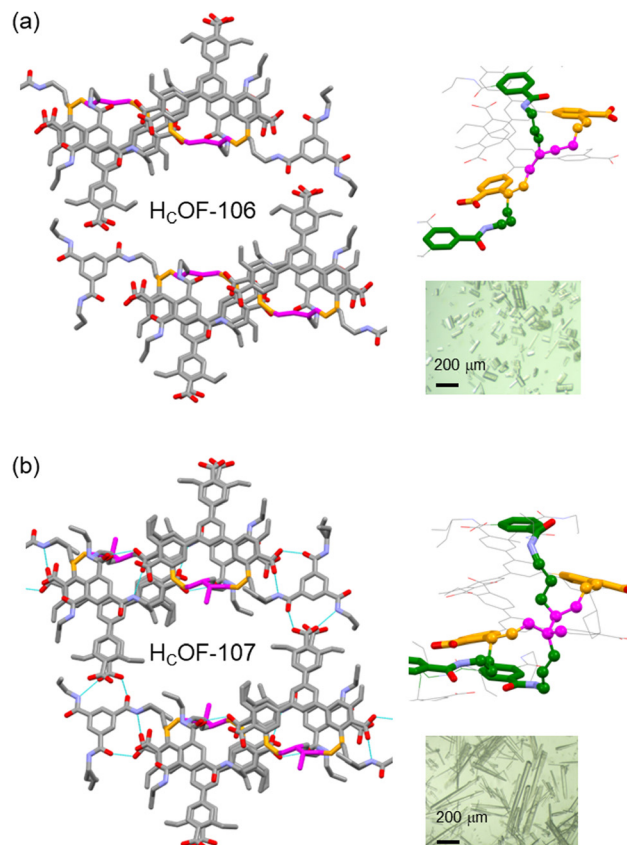
Fig. 3 The SCXRD structure of (a) H c OF-106 and (b) H c OF-107 with highlighted crosslinkers (magenta) in the crystal lattices. The crosslinking connections between the layers in H c OF-106 and H c OF-107 are shown on the right. Inset: Optical images of these crystals.
