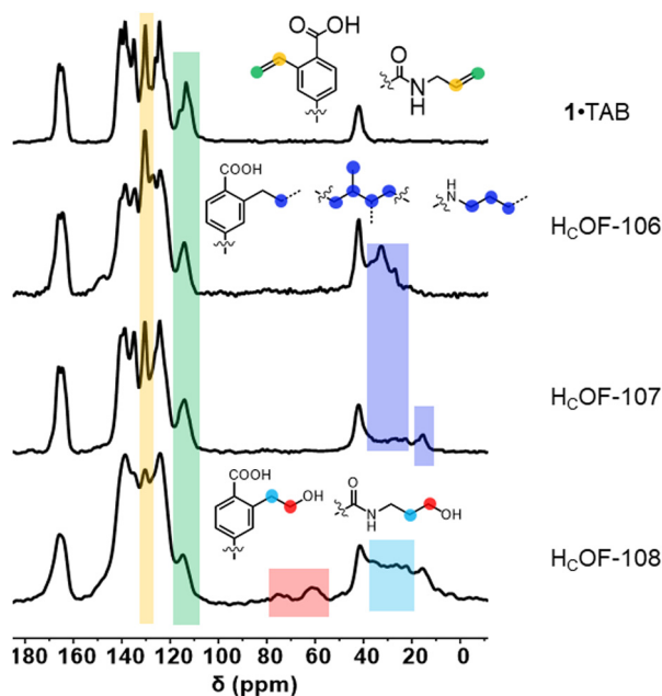
Fig. 2 Stacked solid-state ^{13}\text{C} NMR spectra of 1 -TAB, H c OF-106, H c OF-107, and H c OF-108 from top to bottom, respectively.
