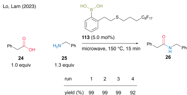
Scheme 24 Fluorous boronic acid-catalyzed amidation reported by Lam. 39
