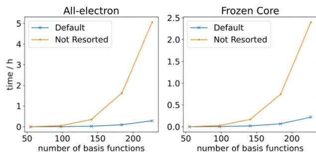
Fig. 1 RHF CCSD 2RDM performance with and without resorting matrix containers. The calculations were performed on linear alkanes of increasing length with a def2-TZVP basis set.
