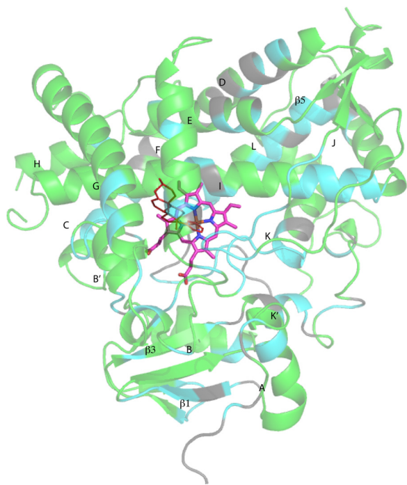
Fig. 3 CYP17A1 (PDB entry 3RUK) with abiraterone bound, showing distribution of sequential backbone resonance assignments. Assignments for regions in green are supported by multiple forms of data (see text for details), regions in blue are provisionally assigned based on fewer data. Those shown in grey are not assigned. Secondary structures were assigned by DSSP analysis of PDB 3RUK (see ESI†) are labeled as first described by Poulos. 23 Helices: A, M49–Y60; B, H80–L86; B', A100–A105; C, A119–A133; D, L142–T159; E, S168–F184; F, E194–L209; G', W120–I123; G, T228–K253; H, M262–N272; I, D289–H320; J, P322–N335; K, L351–L363; K', L396–H401; K'', P414–F417; L, E445–R462. Strands: \beta 1, I63–M68, K71–V76, E391–I394, H373–K374; \beta 2, S379–I381, F384–386; \beta 3, F463–E466, K492–V495; \beta 4, I479–P480, F484–L385; \beta 5, F463–Q466, V491–495. Abiraterone is shown in thin red lines, heme is shown in heavier pink lines.
