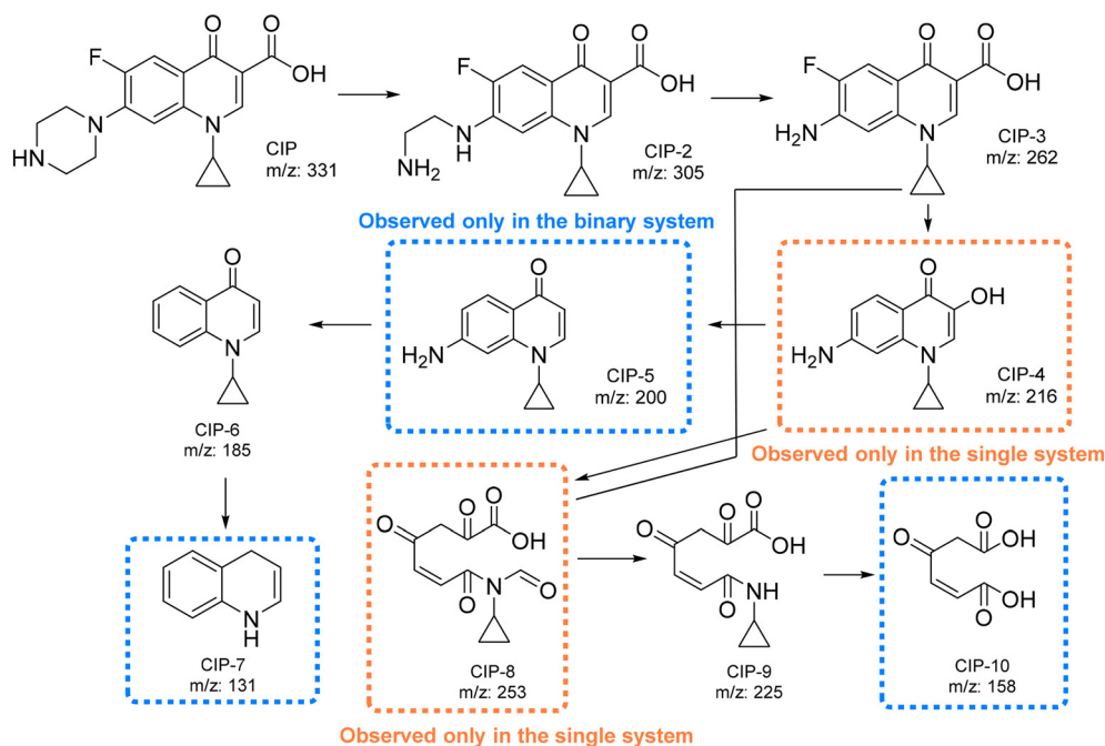
Fig. 13 Proposed pathways for the degradation of CIP using \text{BiOCl}_{0.9}\text{I}_{0.1} in the three different contaminant systems.
