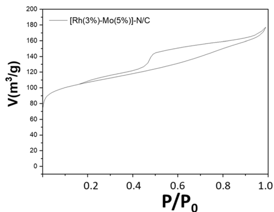
Fig. 9 N 2 -physorption isotherms at -196 °C of the prepared bimetallic [Rh(3%)-Mo(5%)]-N/C sample.
