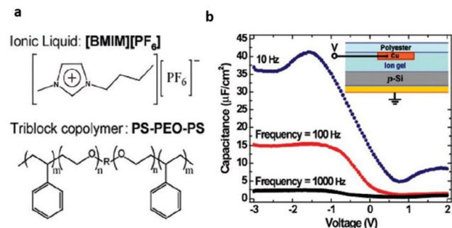
Fig. 7 (a) Structure of the ionic liquid and triblock copolymer ion gel components (b) C - V characteristics of a p -Si/ion gel/Cu test structure (see inset) at three frequencies (right). The C - V curves indicate large frequency-dependent hole accumulation in the Si at negative bias on the top contact. Reproduced from ref. 71 with permission from ACS, Copyright [2007].
