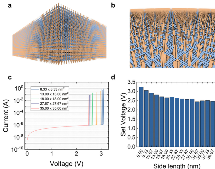
Fig. 5 (a) Resistance network corresponding to a great area (100 nm × 100 nm) device. (b) Resistance network corresponding to a great area (100 nm × 100 nm) device (zoomed-in view). (c) Several simulated set I - V curves for different device areas (the current values are scaled with respect to the lowest area shown in the plot, i.e. (8.33 nm × 8.33 nm)). (d) Set voltage versus device side length (assuming a device square area obtained as (side length) 2 ).
