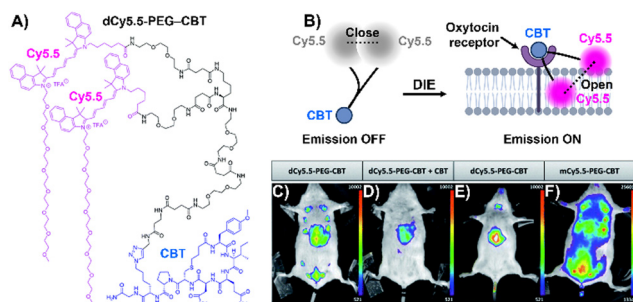
Fig. 12 (A) Chemical structure of dCy5.5-PEG-CBT. (B) Recognition mechanism mediated by dCy5.5-PEG-CBT. (C)–(F) In vivo images of lactating mice (C), (D), and (F) and a naive mouse (E) injected intravenously via the tail with 7.5 nmol of dCy5.5-PEG-CBT (C) and (E), 7.5 nmol of dCy5.5-PEG-CBT along with 450 nmol of CBT (D), or 7.5 nmol of mCy5.5-PEG-CBT (F), taken 30 minutes prior to imaging. Reproduced from ref. 64 with permission from the Royal Society of Chemistry.
