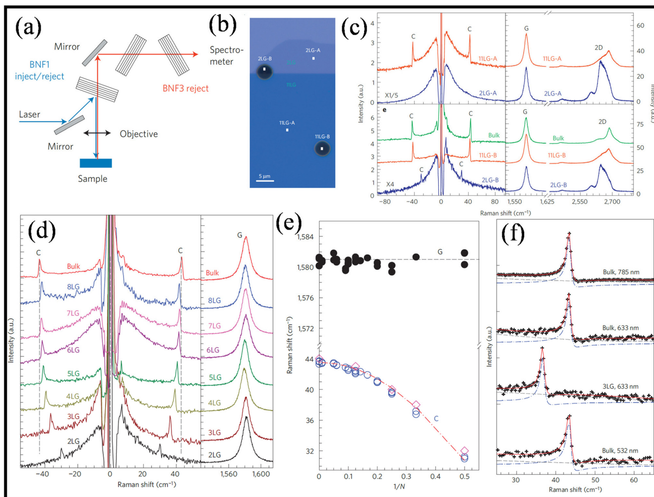
Fig. 7 (a) Schematic diagram of our single monochromator with three BragGrate notch filters (BNF). (b) Optical micrograph of the FLG sample. 2LG-A/11LG-A and 2LG-B/11LG-B denote supported and suspended flakes, respectively, (c) S/AS spectra of supported flakes and suspended flakes, top and bottom, respectively, in the C peak region (left) and S spectra in the G/2D peaks region (right), (d) S/AS Raman spectra for the C peak spectral region (left) and S Raman spectra for the G peak spectral region (right). (e) Peak positions Pos(G) (filled black circles) and Pos(C) (open blue circles) as a function of inverse layer number, (f) C peaks with BWF fit for bulk graphite and 3LG. Fitted curve (solid red lines); background (dashed lines); BWF component (dash-dotted lines). Reproduced from ref. 45 with permission from [Springer Nature], copyright [2012].
