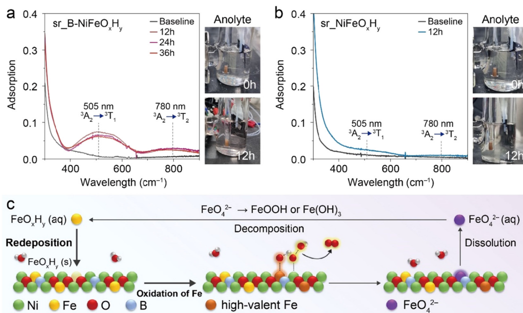
Fig. 3 Detection of Fe VI O 4 2- species using in situ UV-vis spectroscopy of the anolyte during OER. (a) sr _B-NiFeO x H y , (b) sr _NiFeO x H y . (c) The proposed dissolution/redeposition mechanism for the high-valent Fe species in the sr _B-NiFeO x H y catalyst.
