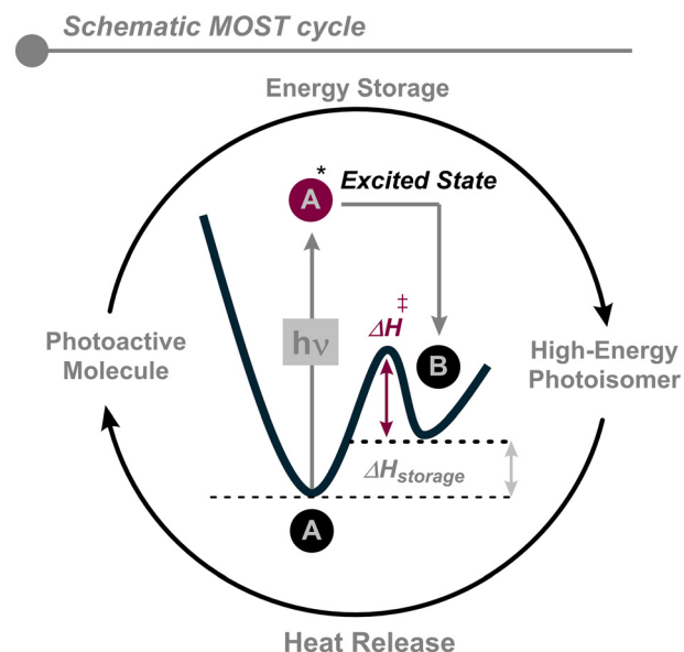
Fig. 1 Schematic representation of photoswitches that behave as MOST systems. A: ground-state isomer. A^* : excited state of the initial isomer. B: meta-stable isomer. \Delta H^\ddagger : thermal activation energy of back conversion.
