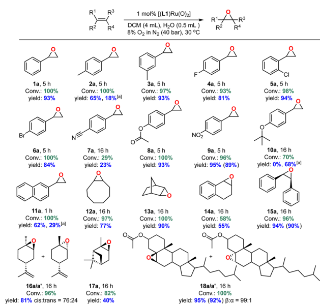
Fig. 13 Substrate scope of [(\text{L1})\text{Ru}^{\text{VI}}(\text{O})_2(\text{H}_2\text{O})_2] catalysed aerobic alkene epoxidation. Conversions and yields determined by quantitative ^1\text{H} NMR spectroscopy against mesitylene as internal standard; isolated yields provided in parentheses. [a] Yield of corresponding aldehyde from epoxide isomerisation.
