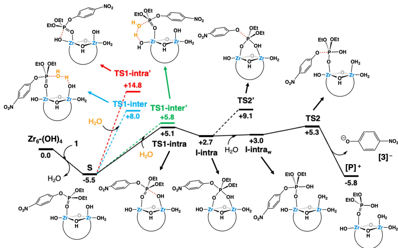
Fig. 7 Gibbs free-energy profile ( \text{kcal mol}^{-1} ) for the hydrolysis of 1 at 60 °C catalyzed by \text{Zr}_6\text{-(OH)}_4 , the most abundant catalytic species at pH 3. Black solid lines represent the lowest free-energy pathway (intra path), while dashed lines denote alternative mechanisms that are higher in energy.
