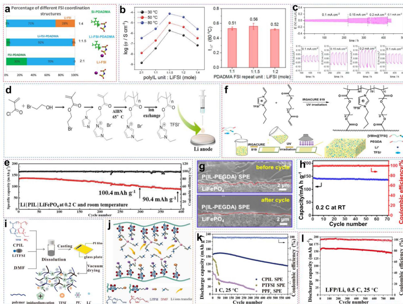
Fig. 10 (a) Percentage of anions in three types of FSI - coordination environment calculated from MD simulations at 353 K. (b) The ion conductivities of different poly(IL)/salt systems at different temperatures and the Li + transference number of solid polymer electrolytes with varying polymer-to-salt ratios. (c) The Li/Li symmetric battery cycling performances of the 1 : 1 polymer electrolyte at various current densities (i.e., 0.1, 0.15, and 0.2 mA cm -2 ). Reproduced from ref. 89 with permission. Copyright 2019, Elsevier. (d) Schematic representation of the synthesis of PIL. (e) Cycling performance of LFP/PIL/Li batteries at 0.2C and RT. Reproduced from ref. 90 with permission. Copyright 2023, The Royal Society of Chemistry. (f) Schematic diagram of the P(IL-PEGDA) SPE copolymerization reaction and preparation process. (g) SEM image of the interface between the LFP cathode and P(IL-PEGDA) SPE before and after 50 cycles. (h) Cycling performance of LFP/P(IL-PEGDA) SPE/Li batteries at 0.2C and RT. Reproduced from ref. 91 with permission. Copyright 2020, American Chemical Society. (i) Schematic illustration of the fabrication of solid polymer electrolytes. (j) Schematic representation of Li + transfer in robust-flexible CPIL SPE. (k) Cycling performance of NCM811/CPIL SPE/Li batteries at 1C and RT. (l) Cycling performance of LFP/CPIL SPE/Li batteries at 0.5C and RT. Reproduced from ref. 84 with permission. Copyright 2024, Elsevier.
