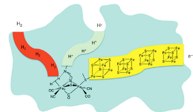
Fig. 1 Depiction of hydrogenase enzyme emphasizing channels for proton, electron and H 2 transport. Fe d and Fe p represent distal and proximal Fe atoms, respectively. 17–20
