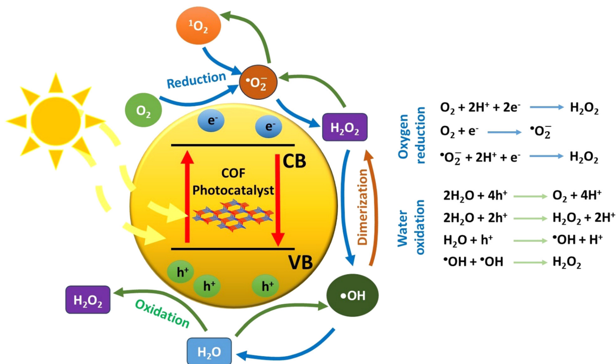
Fig. 1 Underlying mechanistic pathways of reactive oxygen species-mediated processes.
