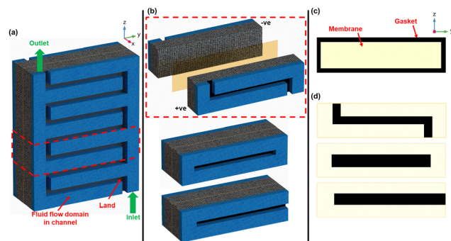
Fig. 2 (a) 3D cell fluid-flow domain with sample interdigitated flow-field. (b) Modeled representative unit of the interdigitated flow-field design (exploded-view) with full membrane coverage and the corresponding variants of parallel and serpentine flow-field designs are shown below. (c) Front view of the representative unit for channel-adjacent membrane reduction. (d) Front view of the representative unit for land-adjacent membrane reduction for; interdigitated, parallel, and serpentine flow-field designs, respectively, vertically stacked.
