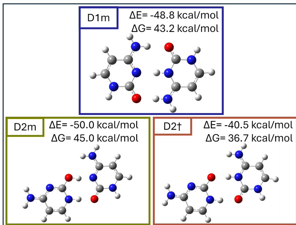
Fig. 5 Optimized structures of the most stable hemiprotonated cytosine dimers in methanol after solvent evaporation and their subsequent rearrangements. D1m and D2m represent D1 and D2 dimers, respectively, optimized in methanol solvent after evaporation. D2† depicts the structure of D2m after rearrangement. Their respective interaction energies ( \Delta E ) and binding free energies ( \Delta G ) with a positive sign indicating stabilization are given above each structure.
