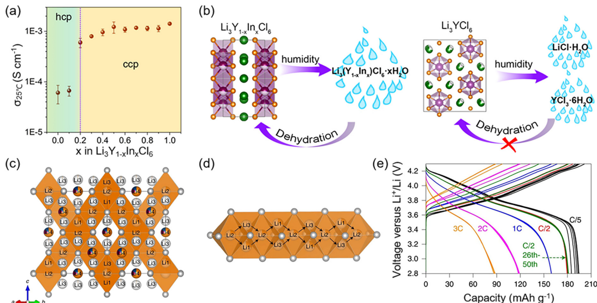
Fig. 7 Influence of isovalent substitution of central metal cation on chemical/electrochemical stability. (a) \text{Li}^+ conductivity at 25^\circ\text{C} for \text{Li}_3\text{Y}_{1-x}\text{In}_x\text{Cl}_6 and corresponding phase transitions. (b) Comparison of humidity stability between \text{Li}_3\text{Y}_{1-x}\text{In}_x\text{Cl}_6 and \text{Li}_3\text{YCl}_6 . Reproduced with permissions from ref. 44. Copyright 2020, American Chemical Society. (c) The main 3D \text{Li}^+ diffusion channels of \text{Li}_2\text{Sc}_{0.666-x}\text{In}_x\text{Cl}_6 . (d) Enlarged pathways of \text{Li}^+ diffusion between tetrahedra and octahedra. (e) Charge-discharge curves of the ASSLB loaded with \text{Li}_2\text{In}_{1/3}\text{Sc}_{1/3}\text{Cl}_6 at different rates. Reproduced with permissions from ref. 30. Copyright 2022, Springer Nature.
