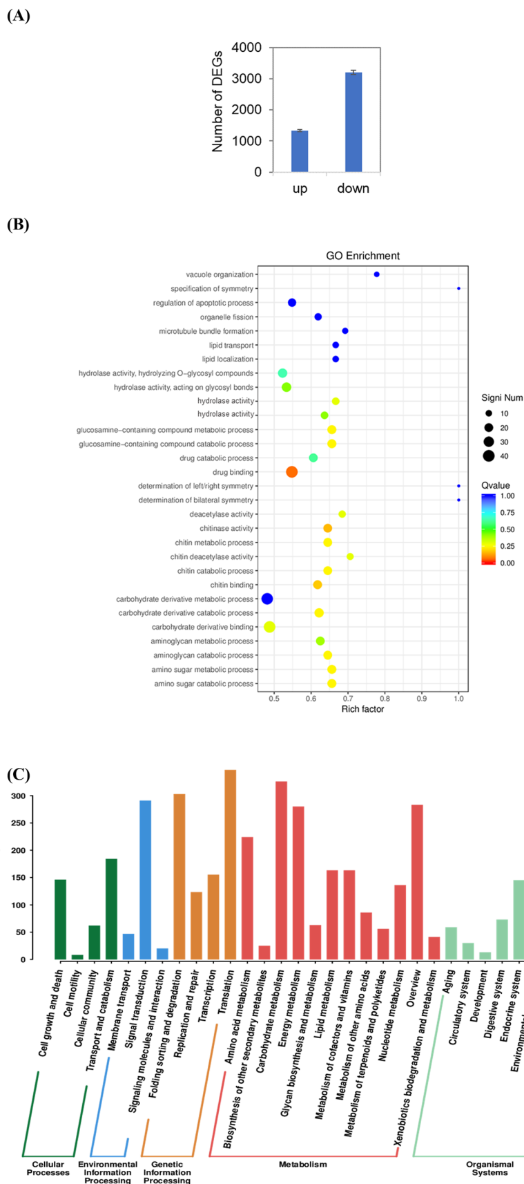
Fig. 6 Transcriptional response of Chlorella vulgaris exposed to ECA-NPs. (A) Number of differentially expressed genes (DEGs) calculated with fold change (ECA-NP exposure/ECA-NP free) \geq 1 and FDR-corrected P -value \leq 0.05 . (B) Biological process GO enrichment of the DEGs. (C) KEGG pathway classification of the DEGs. The cells were harvested for analysis after three-day ECA-NP treatment.
