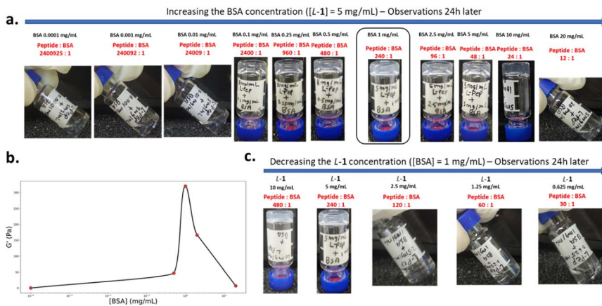
Fig. 5 (a) Inverted vial test realized 24 h after the mixing of L-1 peptide ( 5 \text{ mg mL}^{-1} , PBS 10 \text{ mM} , pH 7.4) with various concentration of BSA. (b) G' values measured by dynamic rheology through a cone-plan geometry in various BSA concentrations with a constant L-1 peptide concentration of 5 \text{ mg mL}^{-1} . A logarithm scale x-axis is used. The black line is a guide for the eye. (c) Inverted vial test realized 24 h after mixing BSA ( 1 \text{ mg mL}^{-1} ) with various concentrations of L-1 peptide.
