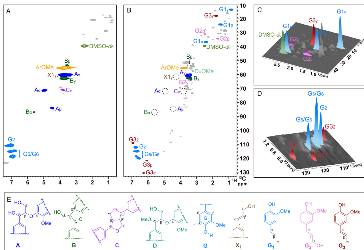
Fig. 6 Characterization of pine lignin and oily products. (A) 2D HSQC NMR spectrum of double enzymatic lignin (DEL) isolated from pine wood (dissolved in \text{DMSO}-d_6 ). (B) 2D HSQC NMR spectrum of the oily product from the Pd–Zn@CN reaction (dissolved in \text{DMSO}-d_6 ). (C and D) 3D version of the HSQC end-chain and aromatic regions. (E) Main structures presented in the 2D HSQC NMR spectra: (A) \beta -O-4' alkyl-aryl ether, (B) \beta -5' phenylcoumaran, (C) \beta - \beta' resinol, (D) \alpha -OH with methylated \beta -O-4' alkyl-aryl ether, (G) guaiacyl units, (X1) cinnamyl alcohol end-groups, (G1) dihydroeugenol, (G2) dihydroconiferyl alcohol, and (G3) isoeugenol.
