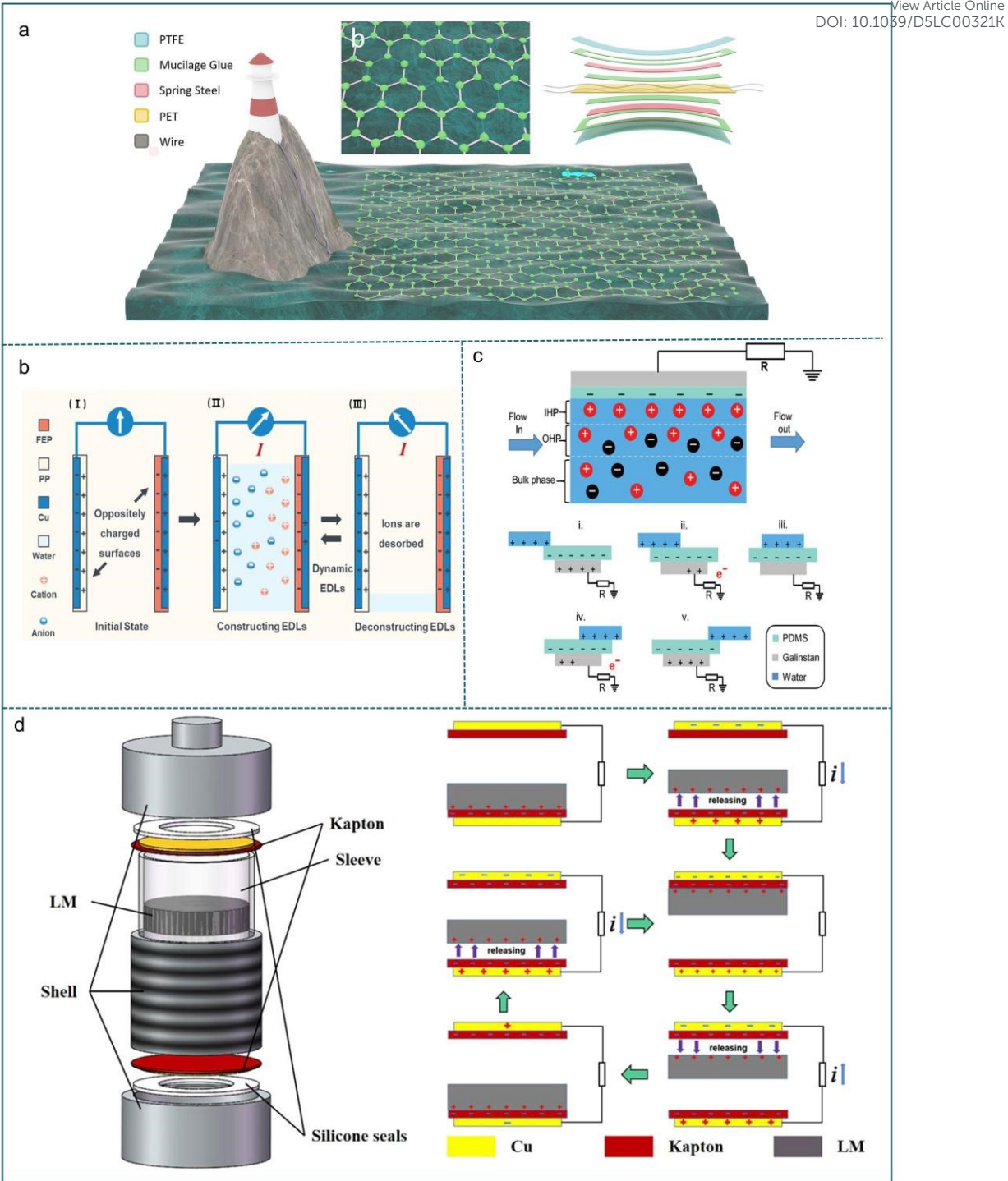
Figure 16. Bulk liquid based generator. a) Illustration of the OS-TENG structure and its potential for large-scale ocean wave energy harvesting. Reproduced with permission. 249 Copyright 2020, Elsevier. b) Asymmetric plate structure of the dielectric layer-based TENG. Reproduced with permission. 185 Copyright 2023, Wiley-VCH GmbH. c) Schematic of liquid metal-TENG harvesting energy through continuous water flow in and out. Reproduced with permission. 250 Copyright 2023, Wiley-VCH GmbH. d) Liquid-metal-based TENG optimized for low-frequency and multidirectional vibrations. Reproduced with permission. 184 Copyright 2021, Frontiers Media S.A.
