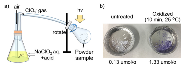
Fig. 3 (a) Schematic image of experimental method PLA powder oxidation. (b) Photographs of untreated and oxidized PLA powder with TBO staining and the values of oxidation degree estimated by TBO treatment.
