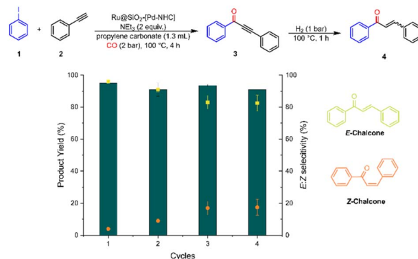
Fig. 7 Recycling experiments for the one-pot synthesis of chalcones 4 using \text{Ru@SiO}_2\text{-[Pd-NHC]} .
