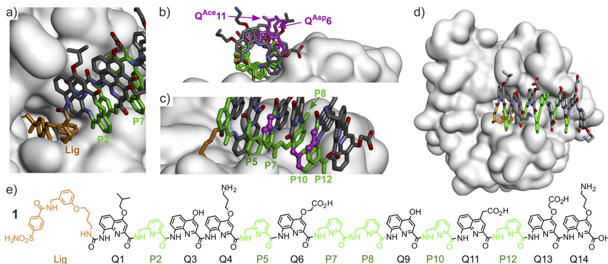
Fig. 2 (a)–(d) Show different views of the solid state structure of the complex between HCAII and AOF 1. 9 Only the surface of the protein is shown. The foldamer is shown in stick representation. Pyridine units (P) are shown in green and the HCAII ligand is shown in gold. In (b), two residues of interest are shown in purple. In (c) three carbon atoms of three P residues are shown in purple balls. These carbons would belong to the additional benzenic ring when implementing a P→Q mutation at these positions. Hydrogen atoms have been omitted for clarity. (e) Structural formula of 1 .
