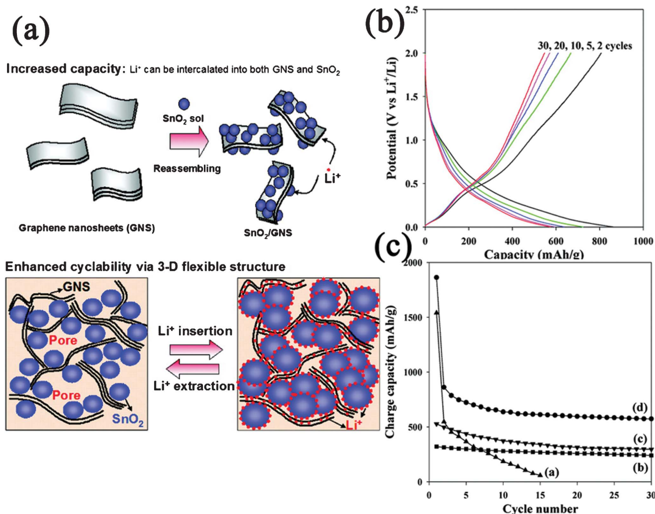
Fig. 13 (a) Schematic illustration for the synthesis and structure change of \text{GN-SnO}_2 nanocomposite during \text{Li}^+ insertion and extraction. (b) Charge-discharge profile for \text{GN-SnO}_2 nanocomposite. (c) Cyclic performances for (a) bare \text{SnO}_2 NPs, (b) graphite, (c) GN, and (d) \text{GN-SnO}_2 nanocomposite. Reprinted with permission from ref. 450. Copyright 2009, American Chemical Society.
