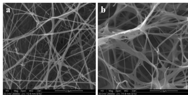
Fig. 3 ESEM images of the surface of a bacterial cellulose membrane cultured for 10 days. (The BC membrane was soaked in water for 2 days and then freeze-dried.)
