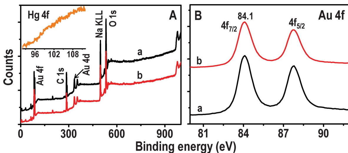
Fig. 7 XPS survey spectra and Au 4f regions (A and B, respectively) of Au@citrate NPs before and after treatment with 5 ppm \text{Hg}^{2+} for 6.0 h (traces a and b, respectively). Inset of A is the Hg 4f region of trace b.
