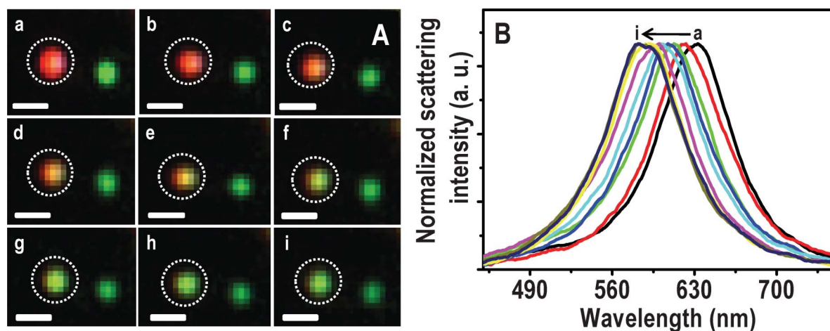
Fig. 2 HSI (A) of immobilized Ag@citrate NPs after passing 5 ppm Hg 2+ for 0.0, 0.5, 1.0, 1.5, 2.0, 2.5, 3.0, 4.0 and 6.0 h (a–i, respectively). Scattering spectra (B) of a red particle with time (a–i). Scale bars of images in A are 500 nm. The particle from which spectra are collected is marked.
