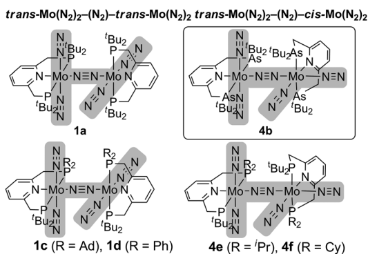
Chart 2 Comparison of structures of dinitrogen-bridged dimolybdenum-dinitrogen complexes.
