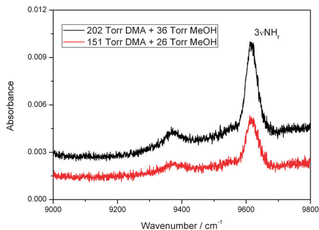
Fig. 3 The 3\tilde{\nu}_{\text{NH}_t} band of the MeOH–DMA complex obtained by spectral subtraction of 202 Torr DMA and 36 Torr MeOH from the mixture of the two gases (upper trace), and of 151 Torr DMA and 26 Torr MeOH from the mixture of the two gases (lower trace). The spectra were recorded in a 4.8\text{ m} path length cell using an NIR light source and an InGaAs detector at 297\text{ K} .
