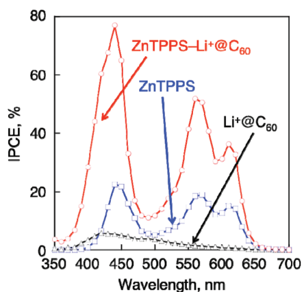
Fig. 6 Photocurrent action spectra of OTE/SnO 2 /(ZnTPPS 4- /Li + @C 60 ) n (red) OTE/SnO 2 /(ZnTPPS 4- ) n (blue) and OTE/SnO 2 /(Li + @C 60 ) n (black). Electrolyte: 0.5 M I 2 and 0.01 M I 3 - in MeCN–PhCN (3 : 1 v/v).
