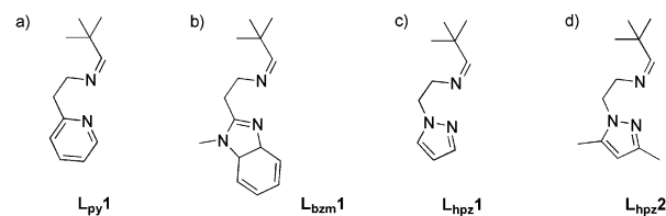
Scheme 2 (a) Ligand \text{L}_{\text{py}}\text{1} of the first mononuclear catalytic model system, (b) ligand \text{L}_{\text{bzm}}\text{1} and ligands \text{L}_{\text{hpz}}\text{1} and \text{L}_{\text{hpz}}\text{2} of this study (c and d). 11,21
