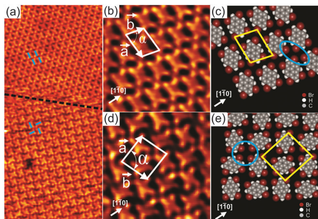
Fig. 1 (a) Overview STM image ( 30 \times 14 \text{ nm}^2 ) for 1 ML \text{Br}_4\text{Py} on \text{Au}(111) , showing the co-existence of two different molecular arrangements, labelled phase I (top) and phase II (bottom). (b, c) and (d, e) Close-up STM images ( 5 \times 5 \text{ nm}^2 ) and corresponding proposed molecular models for phase I and II, respectively. The STM images were taken at room temperature with U = -1.2 \text{ V} , I = 60 \text{ pA} .
