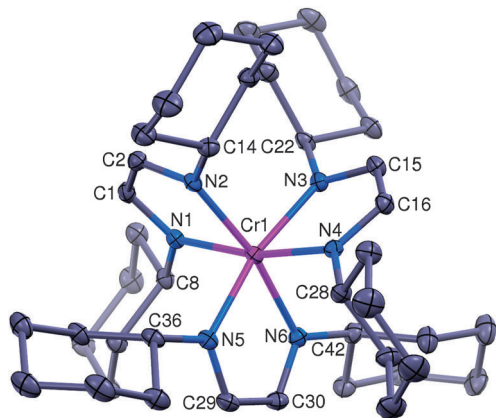
Fig. 1 The structural diagram of the [(^{\text{HLY}})_3\text{Cr}]^{3+} cation ( \mathbf{1}^+ ) at 30% probability. The \text{BARF}^- counterion, one toluene solvent molecule and all hydrogen atoms have been omitted for clarity.
