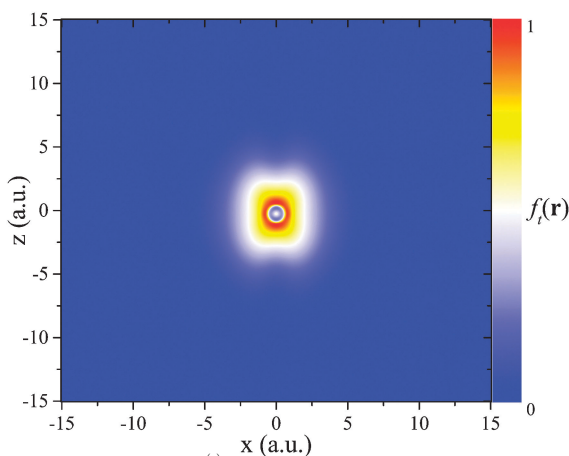
Fig. 5 The LMF f_i(\mathbf{r}) = \frac{1 - \frac{\tau_W(\mathbf{r})}{\tau(\mathbf{r})} c^2}{1 + c^2 \frac{\tau_W(\mathbf{r})}{\tau(\mathbf{r})}} , evaluated with c = 0.5 , on the numerical grid for the C atom.
