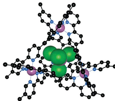
Fig. 16 The encapsulation of [\text{FeCl}_4]^- within a \text{Fe}_4(\mathbf{95})_6 cage, along with the crystal structure of \text{Fe}_4(\mathbf{95})_6 \cdot (\text{FeCl}_4) \cdot (\text{PF}_6)_7 \cdot \text{CH}_3\text{OH} . Iron and [\text{FeCl}_4]^- ions are shown in spacefill with ligand \mathbf{95} in ball-and-stick (iron: purple, chloride: green, nitrogen: blue, carbon: black). Hydrogen atoms, solvent molecules and counterions are omitted for clarity.
