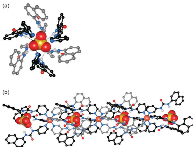
Fig. 6 Crystal structure of the [\text{Cu}^1] fragment in \text{CuSO}_4 complex of 32 . Sulfate and copper ions are shown as spacefill, while the receptor is shown as ball-and-stick. Hydrogen bonds are represented by dashed lines. (a) Sulfate encapsulation by multiple hydrogen bonds from six urea groups in the [\text{SO}_4(\mathbf{32})_6]^{2-} capsule (copper ions are omitted for clarity). (b) Infinite 1D hydrogen bonded chain linked by sulfate encapsulation and copper coordination.
