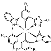
55: \text{R}_1 = \text{H} , \text{R}_2 = \text{'Bu} (fbmb) 2 Ir(bptz)
