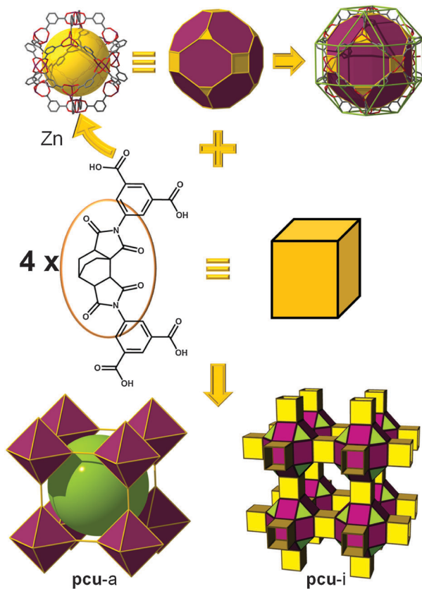
Fig. 24 Quadruple crosslinking of rdo SBB (points of extension defining a rhombicuboctahedron) leads to an SBB-based MOF with pcu-i topology.
