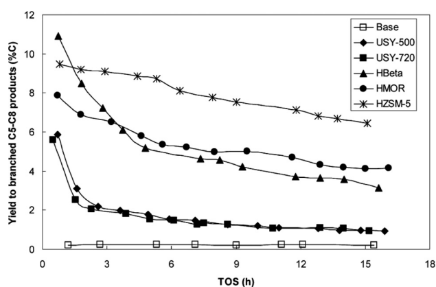
Fig. 17 Yield to branched C 5 -C 8 products (% C) vs. time-on-stream (TOS) for the base and hybrid catalyst in conditions: 250 °C, 20 bar, \text{H}_2/\text{CO} = 2 and 13.5\text{ l}_{\text{syngas}}\text{ g}_{\text{cat}}^{-1}\text{ h}^{-1} . Reprinted with permission from ref. 142, Copyright © 2007, Elsevier.
