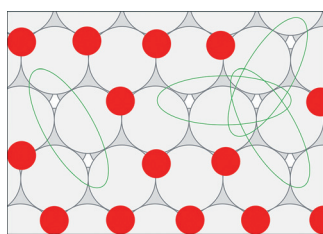
Fig. 6 Reaction sites (ovals) on an oxygen atom equilibrated FCC surface.
