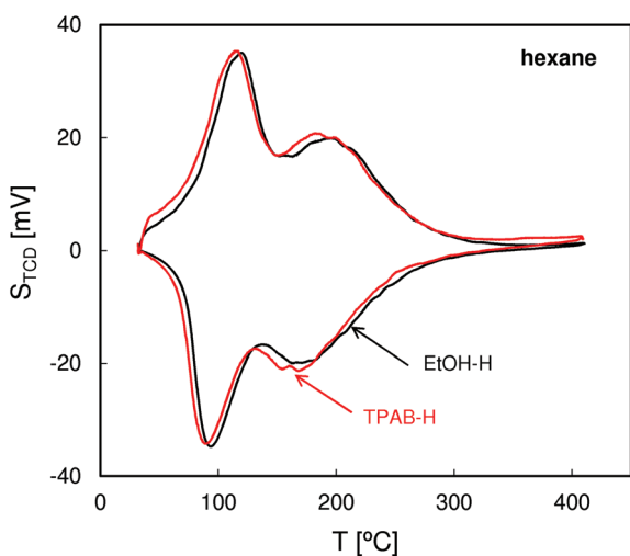
Fig. 4 QE-TPDA profiles of hexane measured for the studied ZSM-5 zeolites at 10\text{ °C min}^{-1} .
