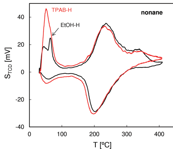
Fig. 5 QE-TPDA profiles of nonane measured for the studied ZSM-5 zeolites at 10\text{ °C min}^{-1} .
