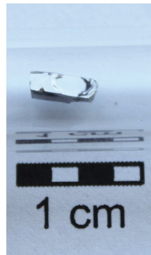
Fig. 1 Example of a bar-shaped single crystal of \text{Li}_{16.38}\text{Ge}_4 obtained from a melt \text{Li}_{85}\text{Ge}_{15} at 530 °C.
